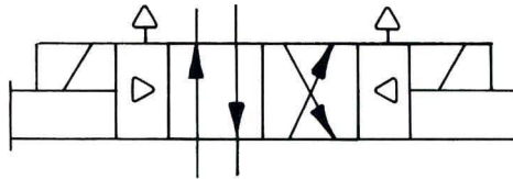
Simplified Symbol
