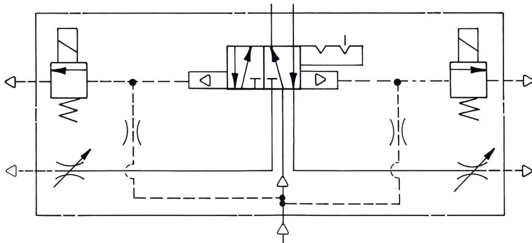
Complete Symbol
