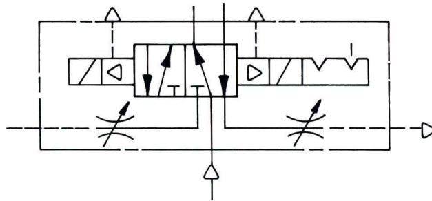
Simplified Symbol
