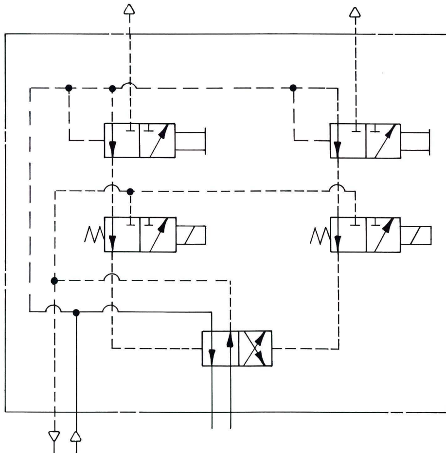
Complete Symbol
